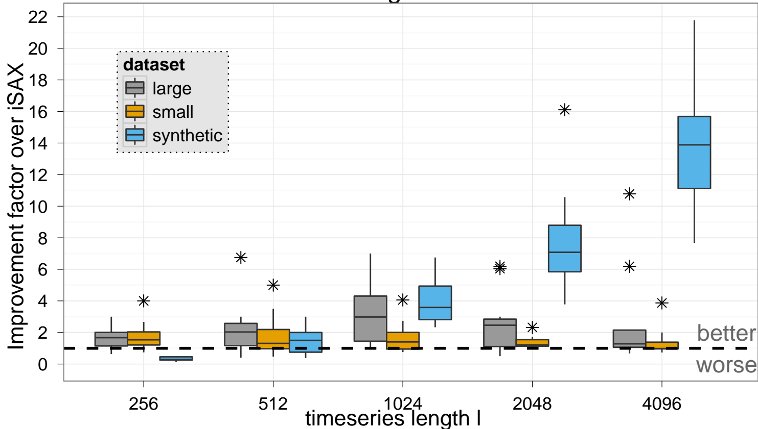
Ratio of wall clock time using SFA trie vs. the iSAX index
